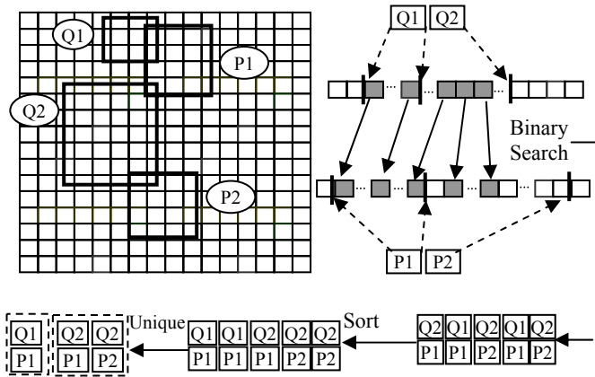
Fig. 4 Illustration of Grid-File based Spatial Join Filtering and its GPU implementation using Parallel Primitives
